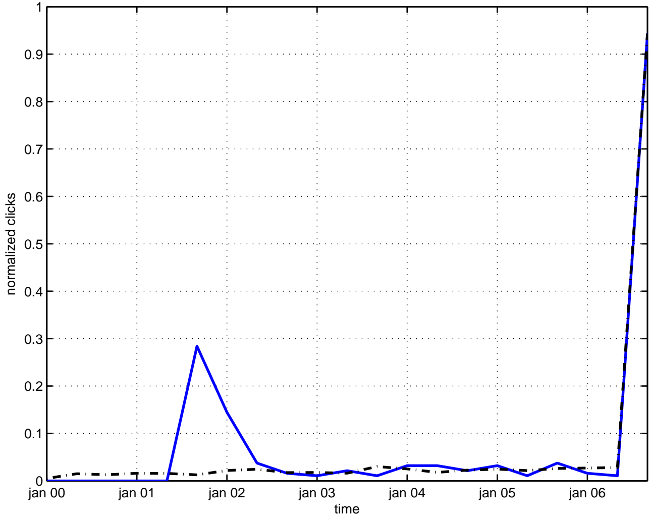
bound state magnetic monopole
