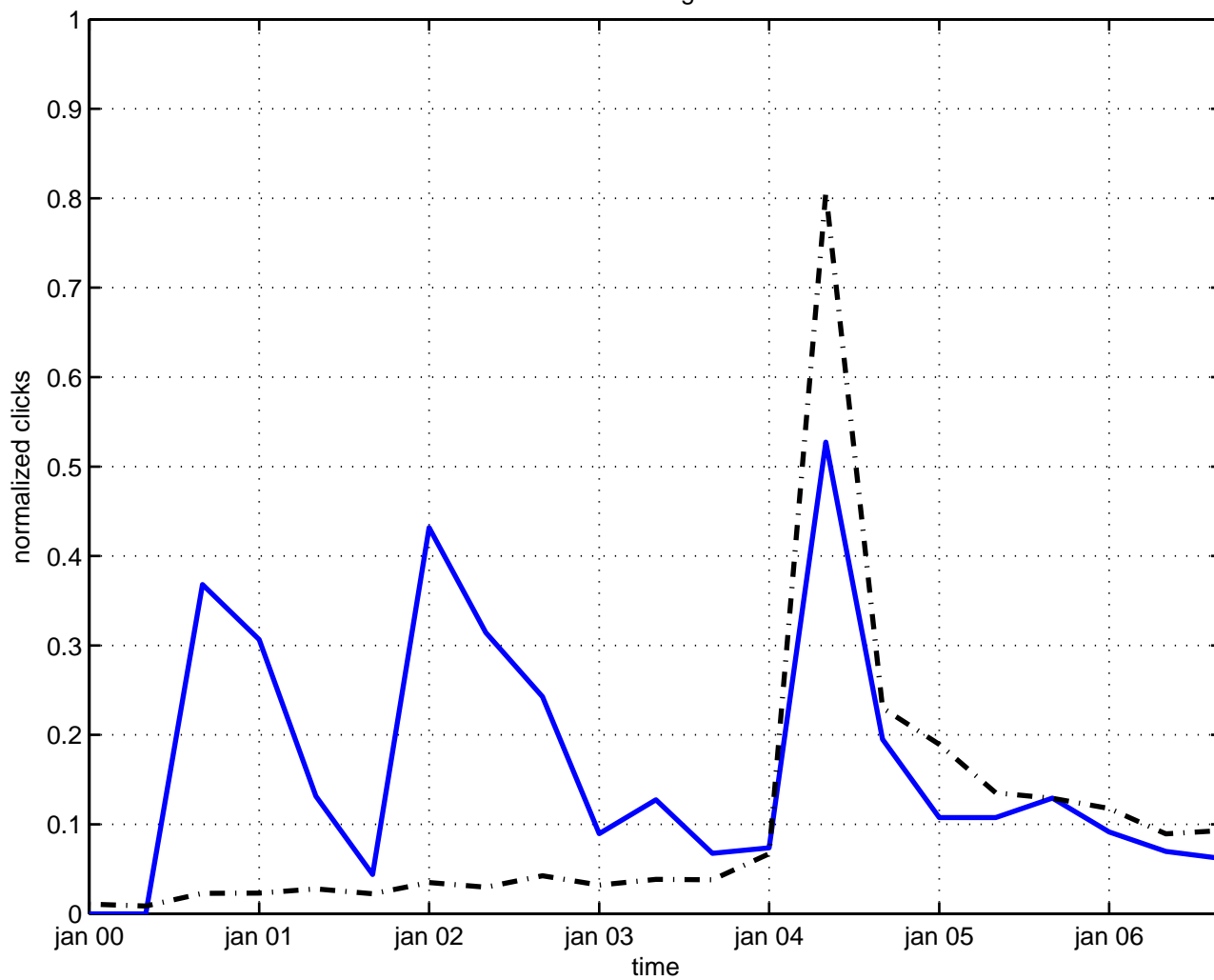
bound state graviton
