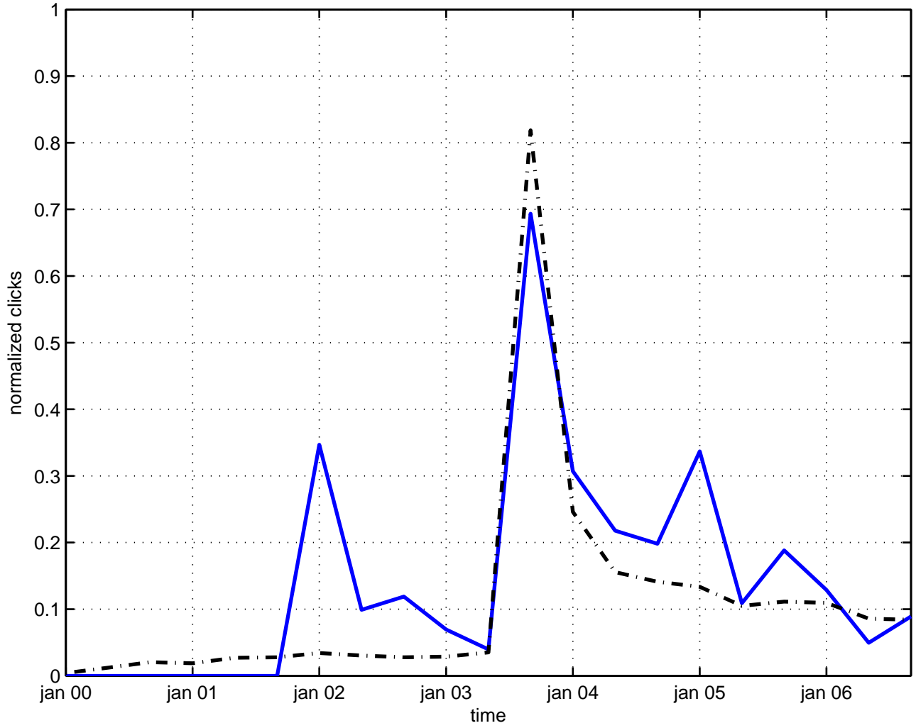
bound state fermion antifermion
