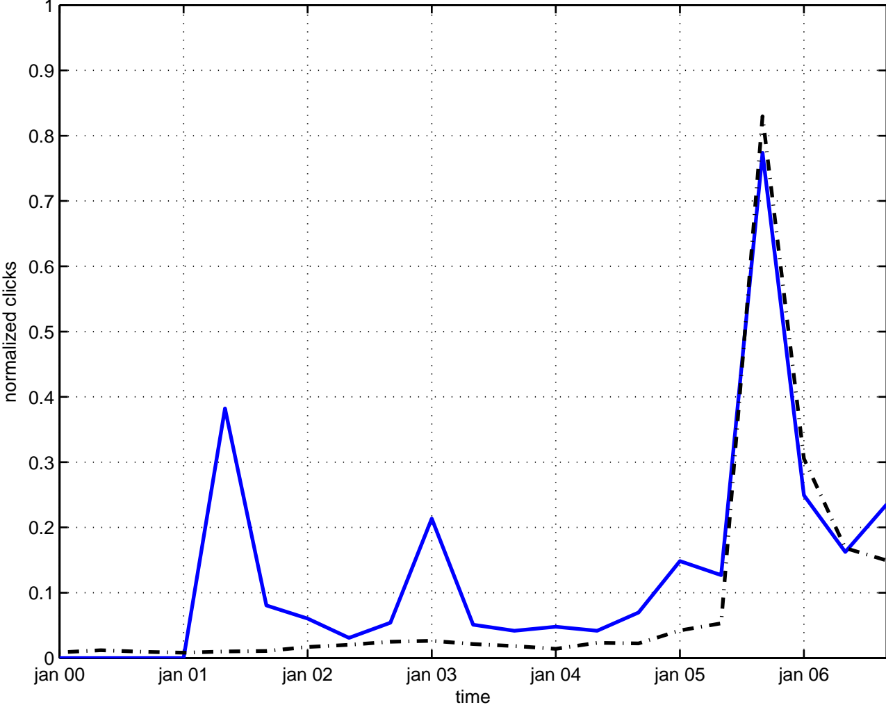
bound state black hole
