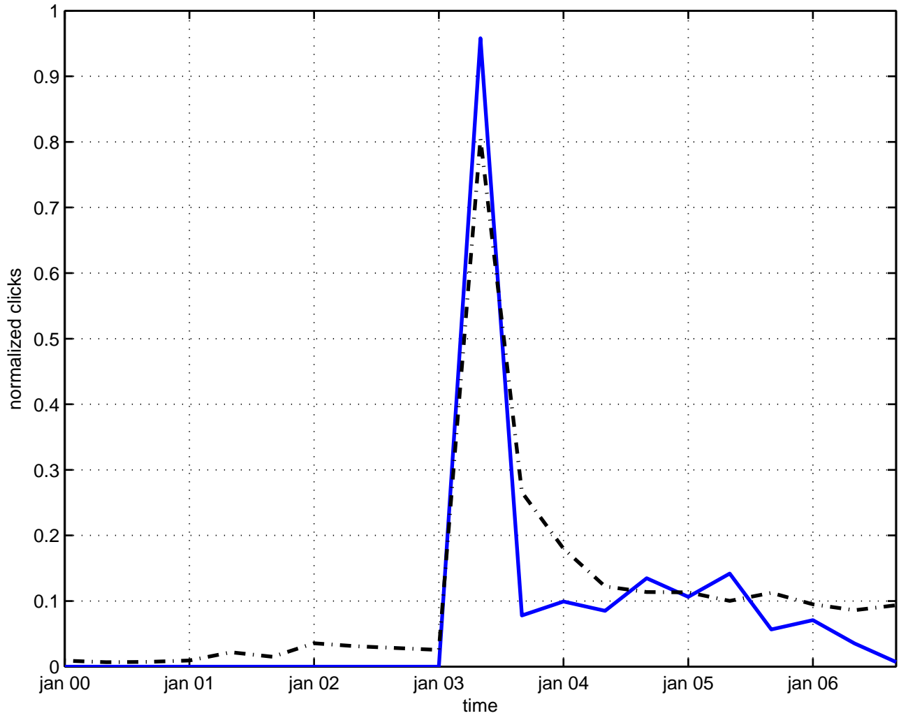
bounce astrophysics
