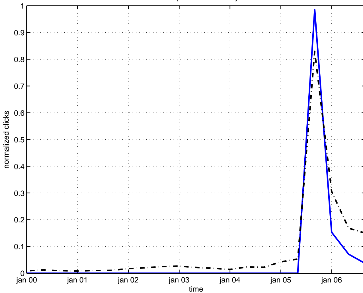
bosonization quantum chromodynamics
