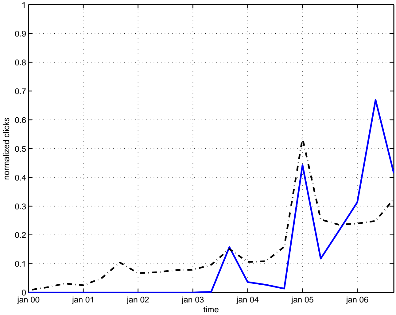
bose-einstein condensation
