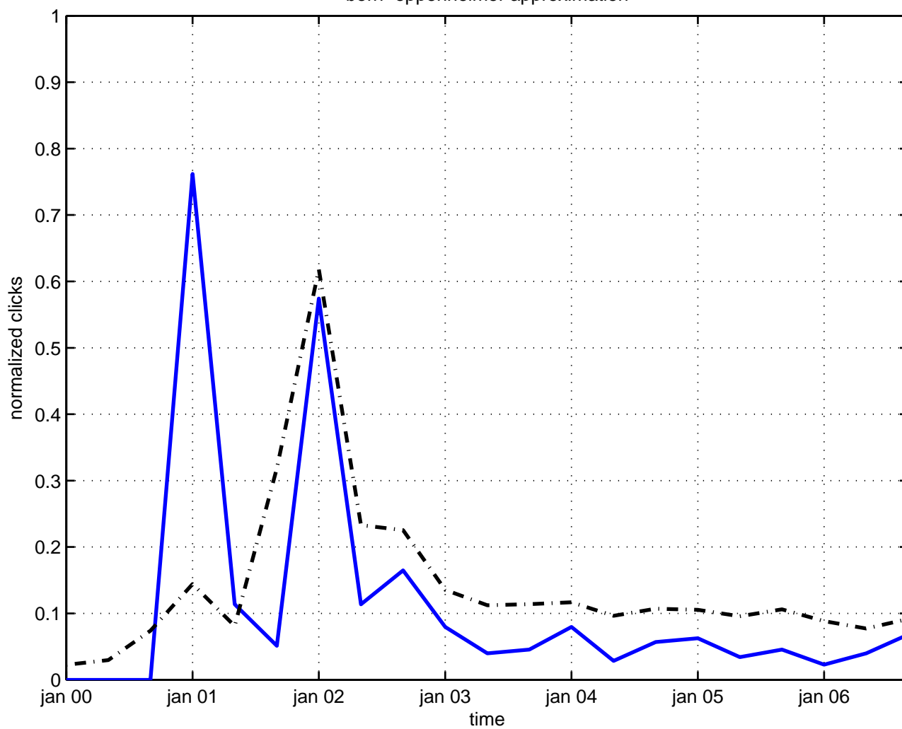
born–oppenheimer approximation
