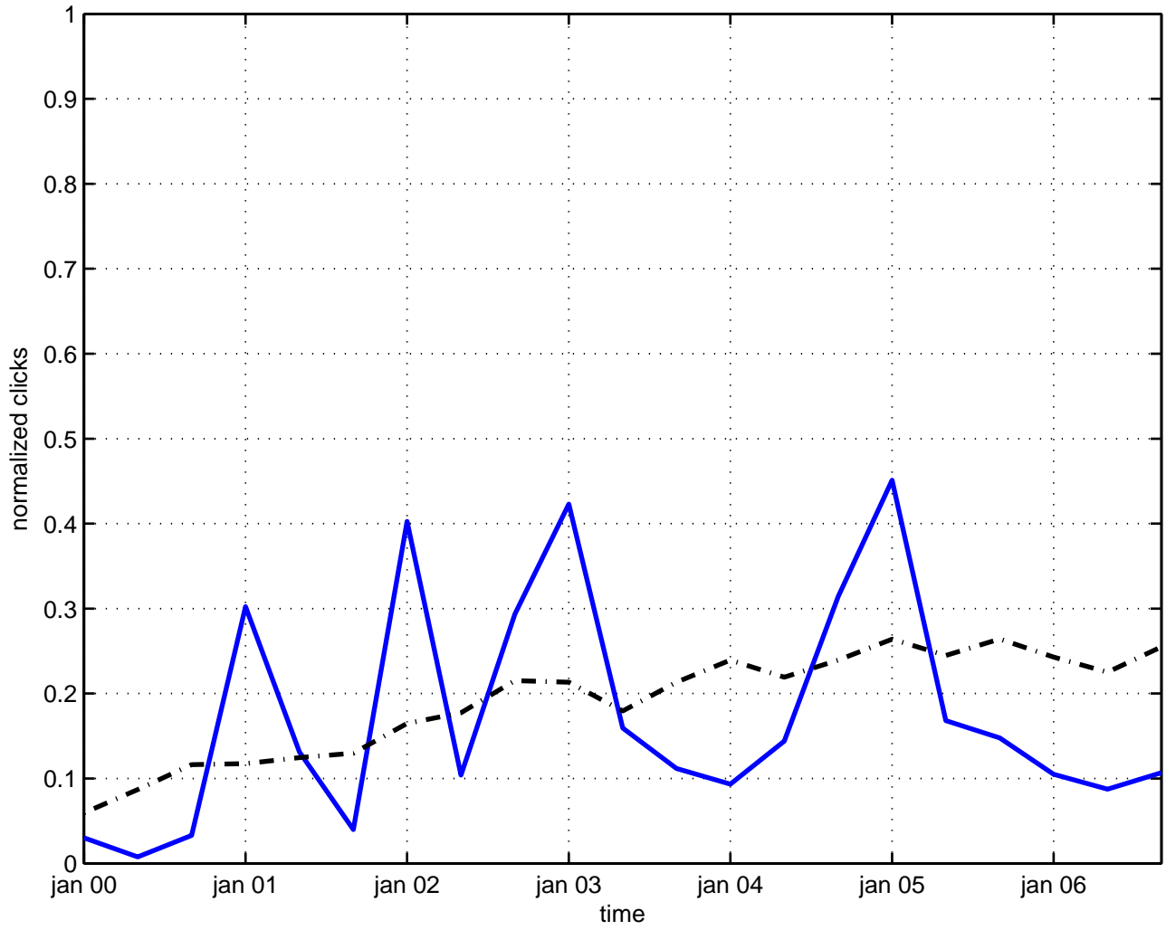
born approximation
