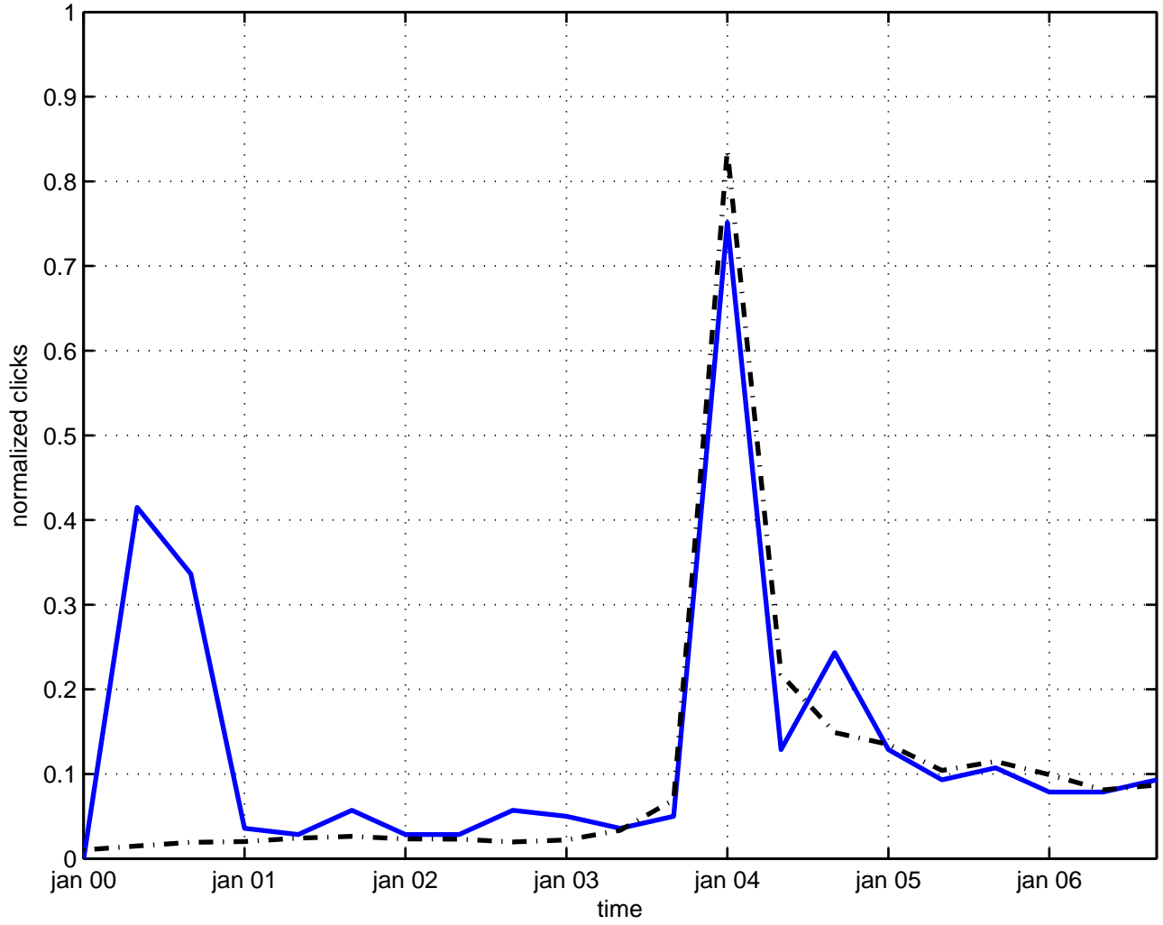
borel transformation
