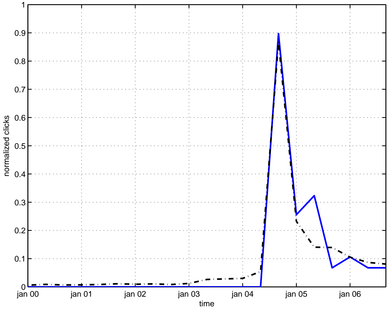
bondi-metzner-sachs group theory
