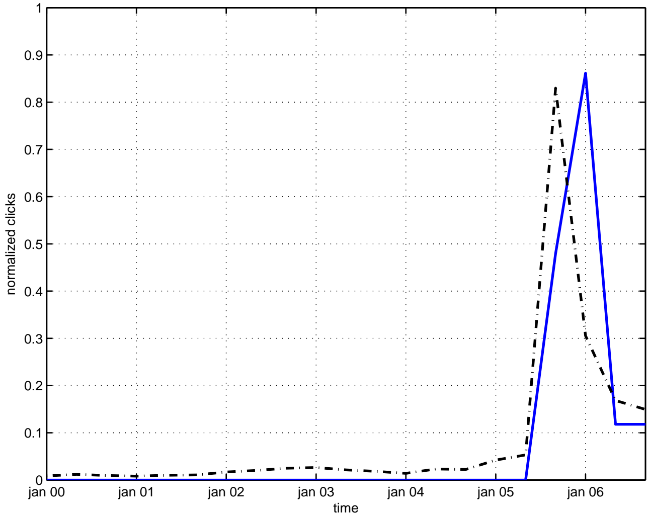
bondi dipole
