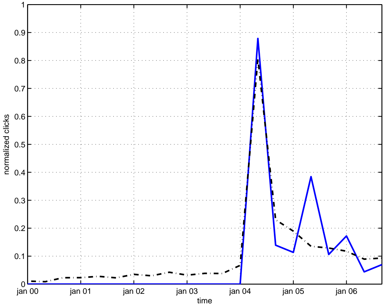
bohm mechanics
