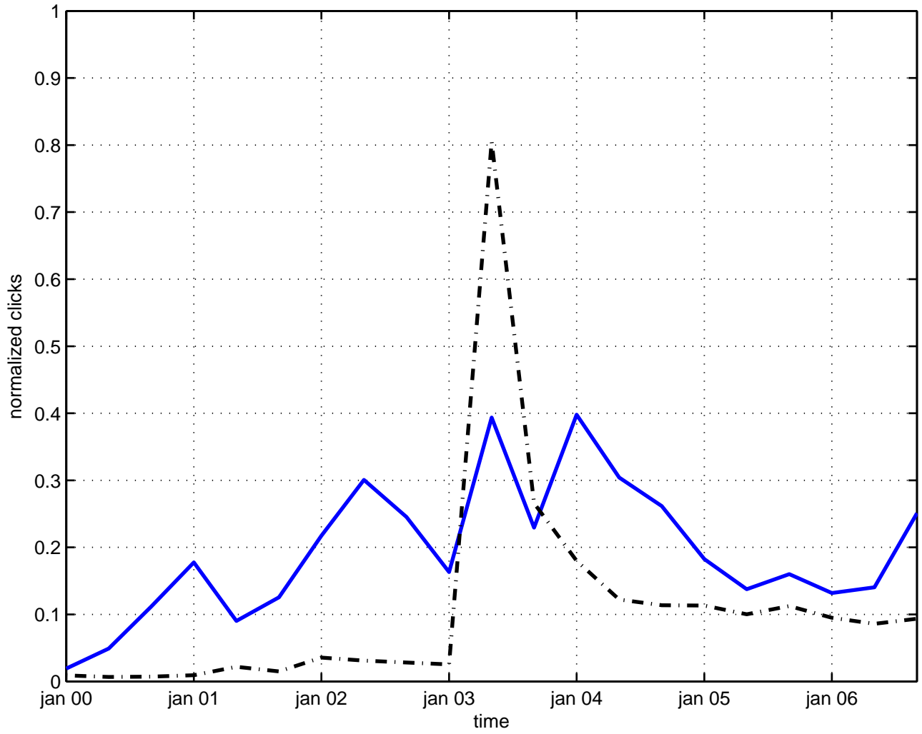
bogolyubov transformation
