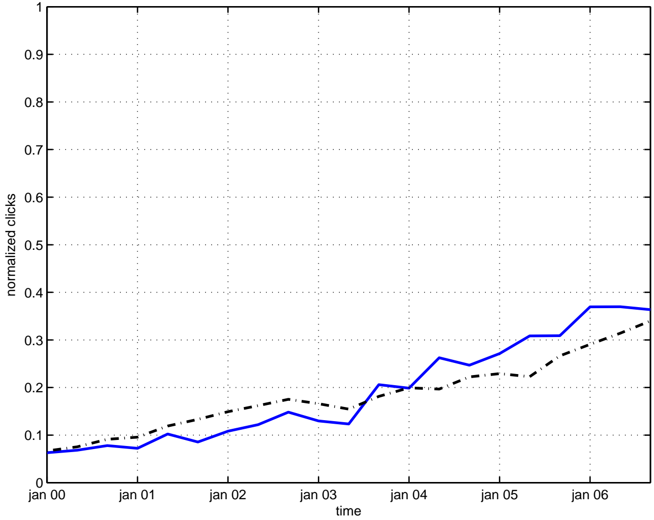
black hole
