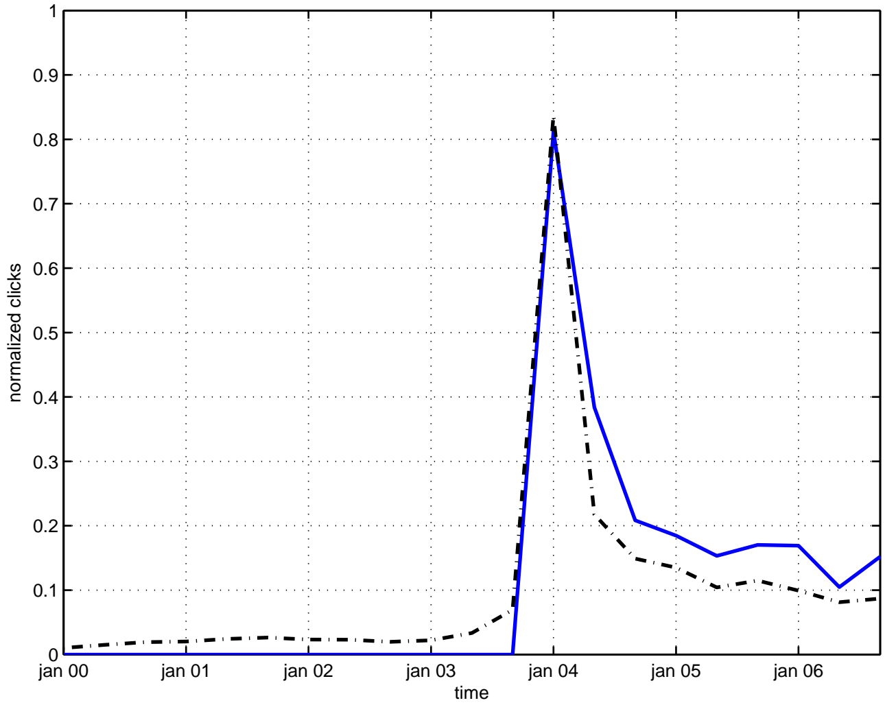
birkhoff theorem
