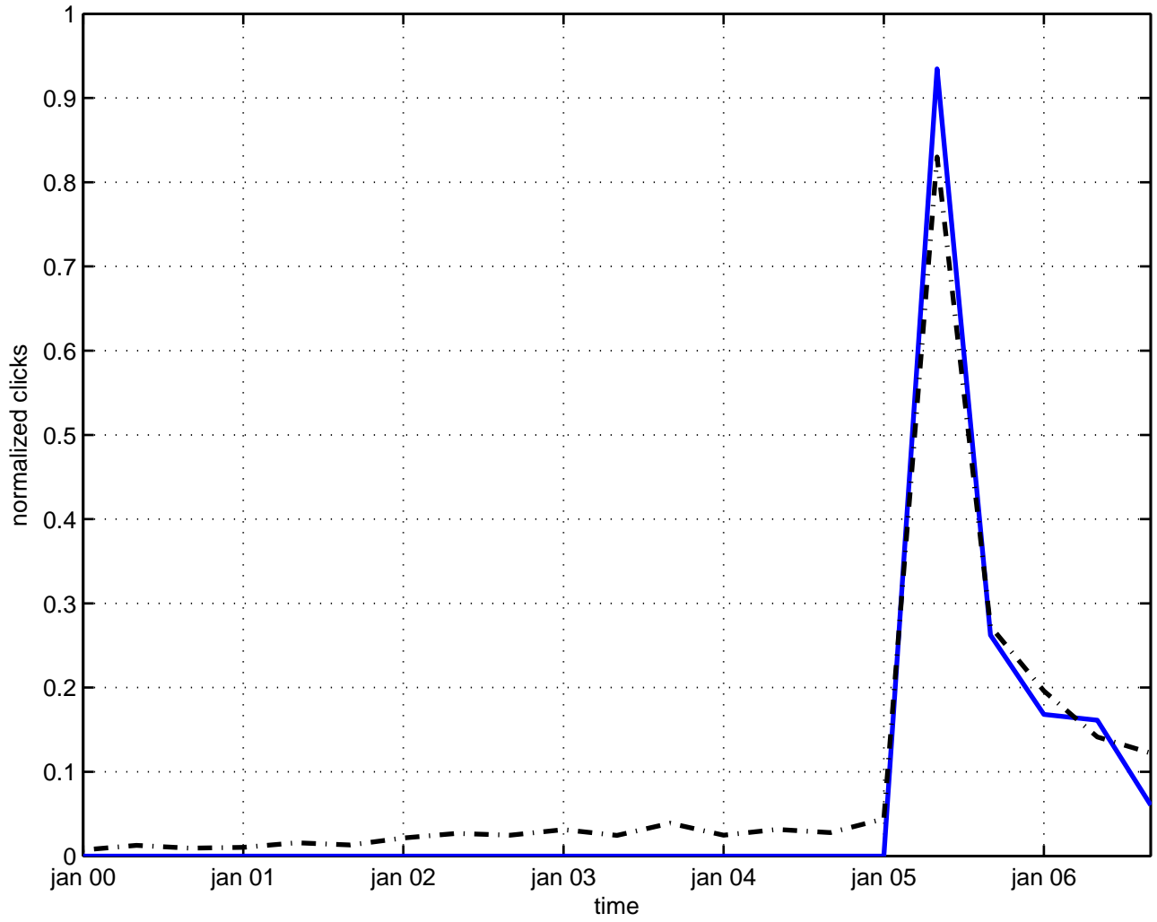
big rip singularity
