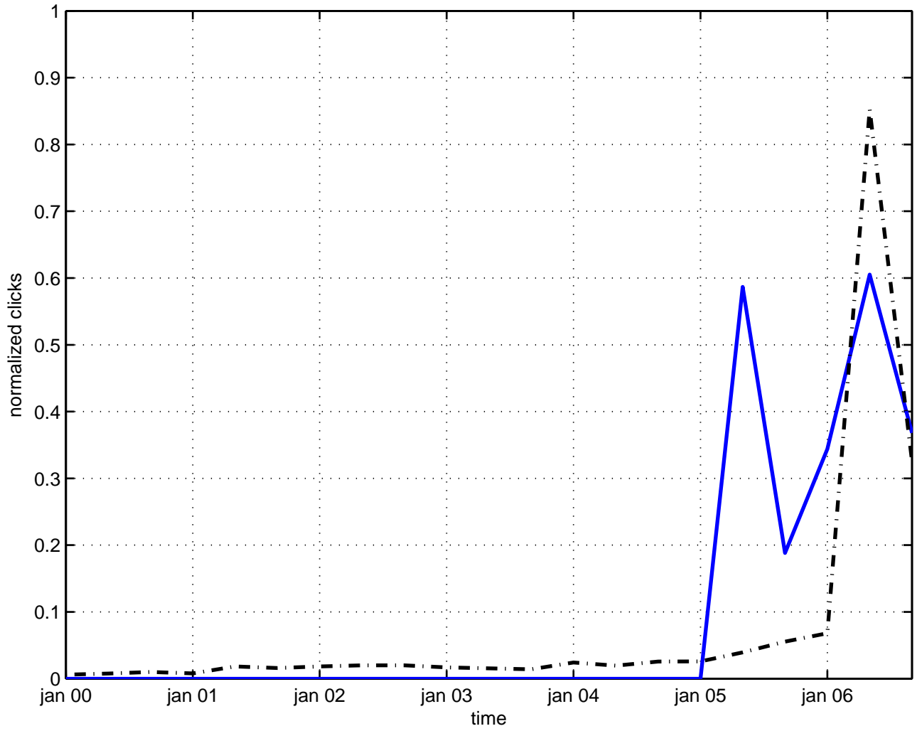
big bang
