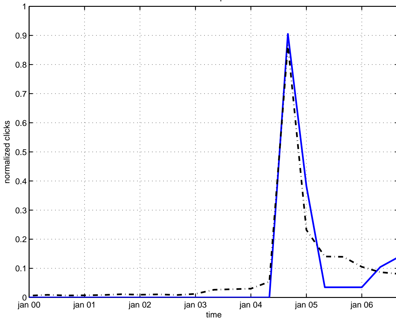
bifurcation sphaleron
