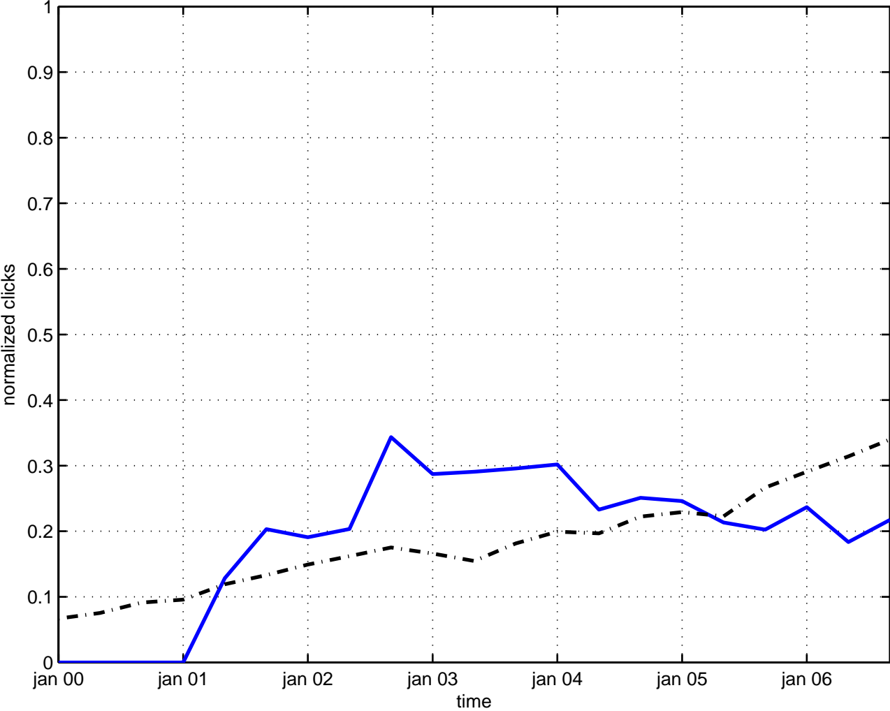
bianchi identity gauge field theory
