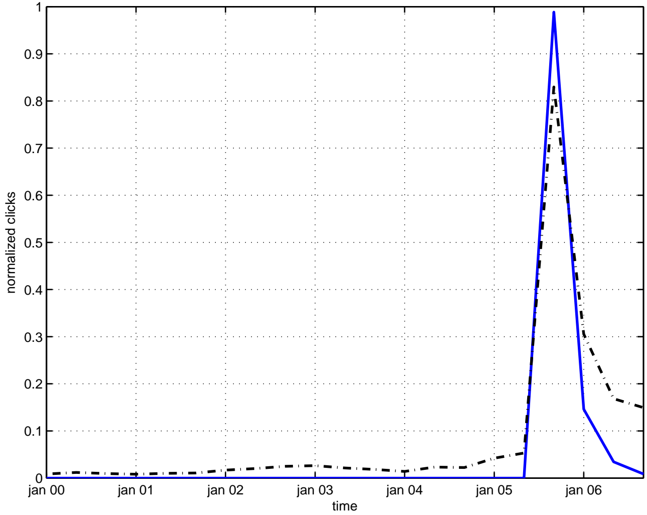
beta function quantum chromodynamics
