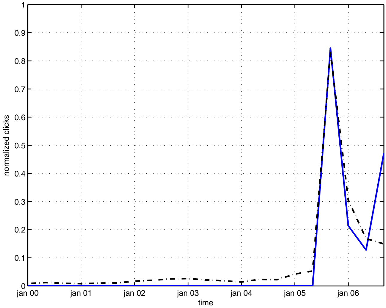
becchi-rouet-stora soliton
