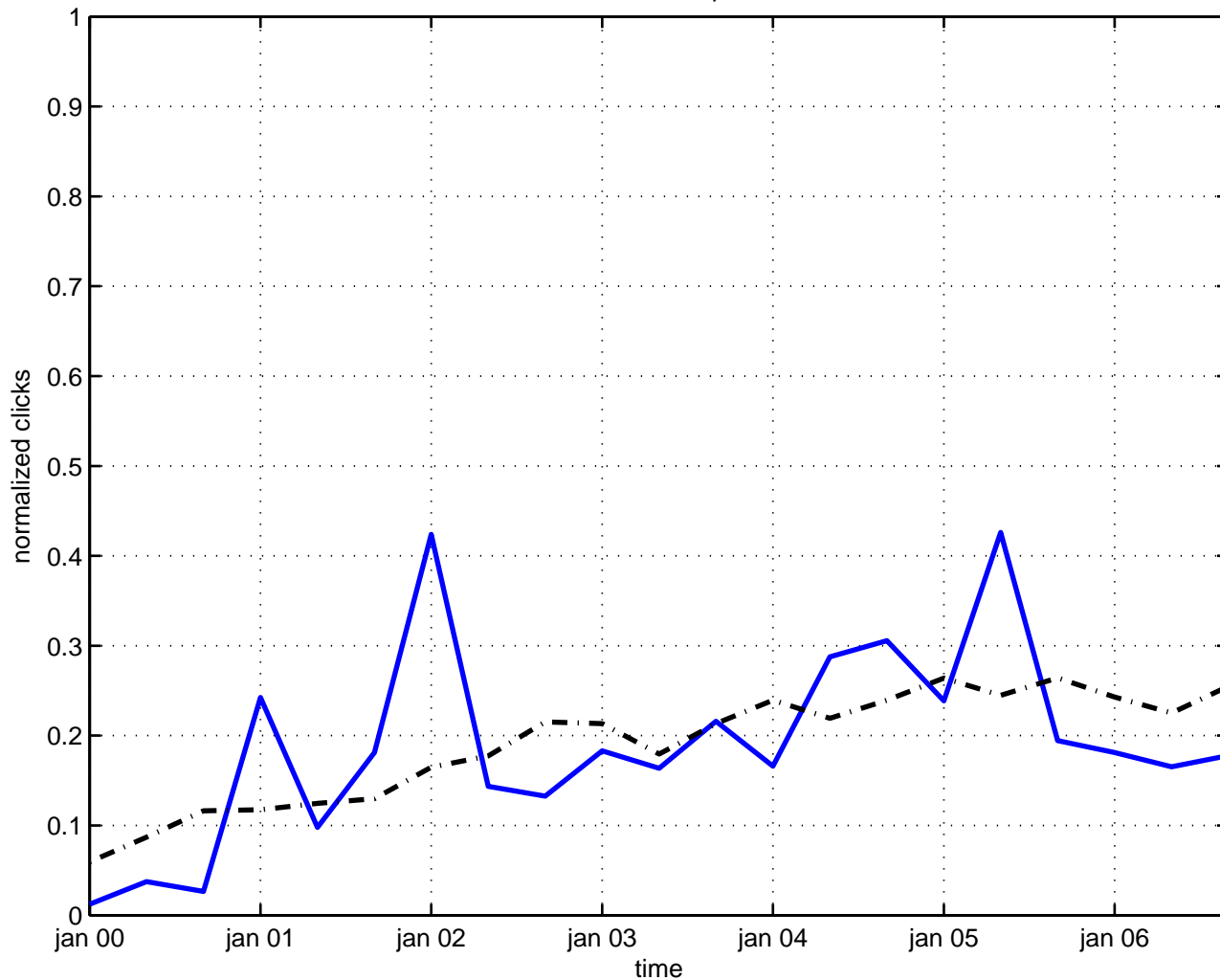
becchi-rouet-stora quantization
