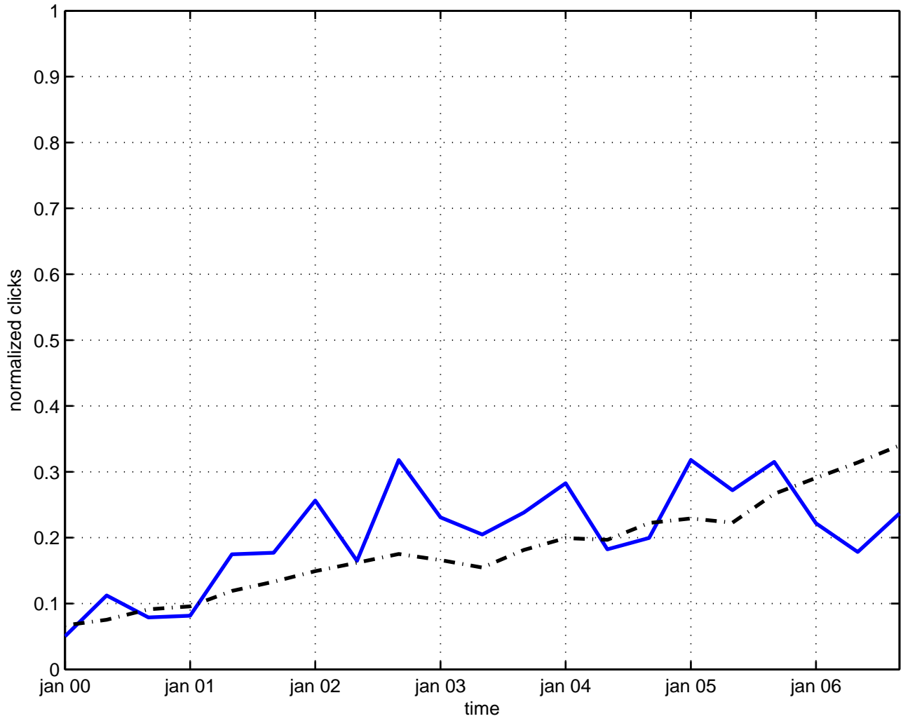
becchi-rouet-stora invariance
