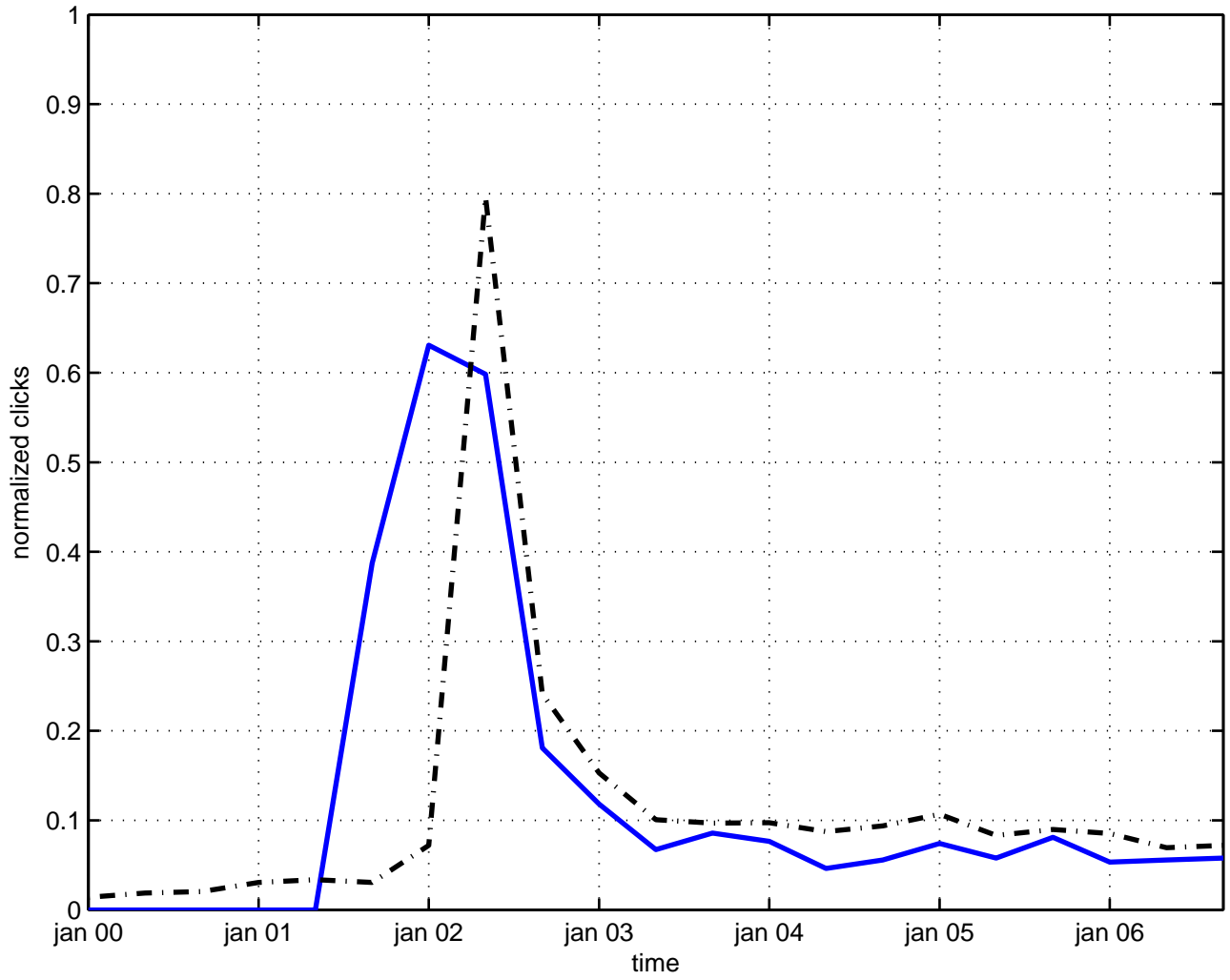
becchi-rouet-stora current
