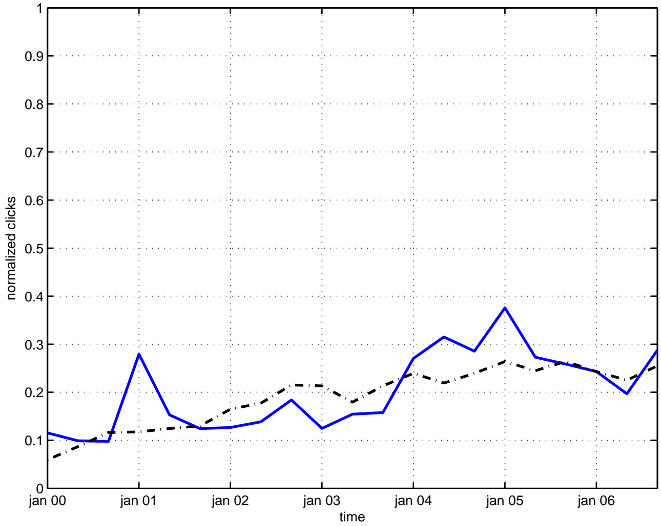
becchi-rouet-stora cohomology
