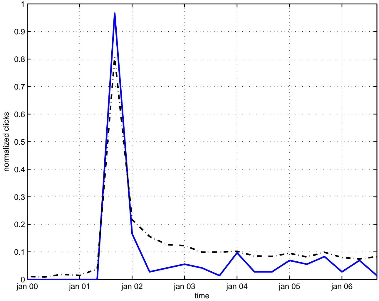
becchi-rouet-stora anomaly
