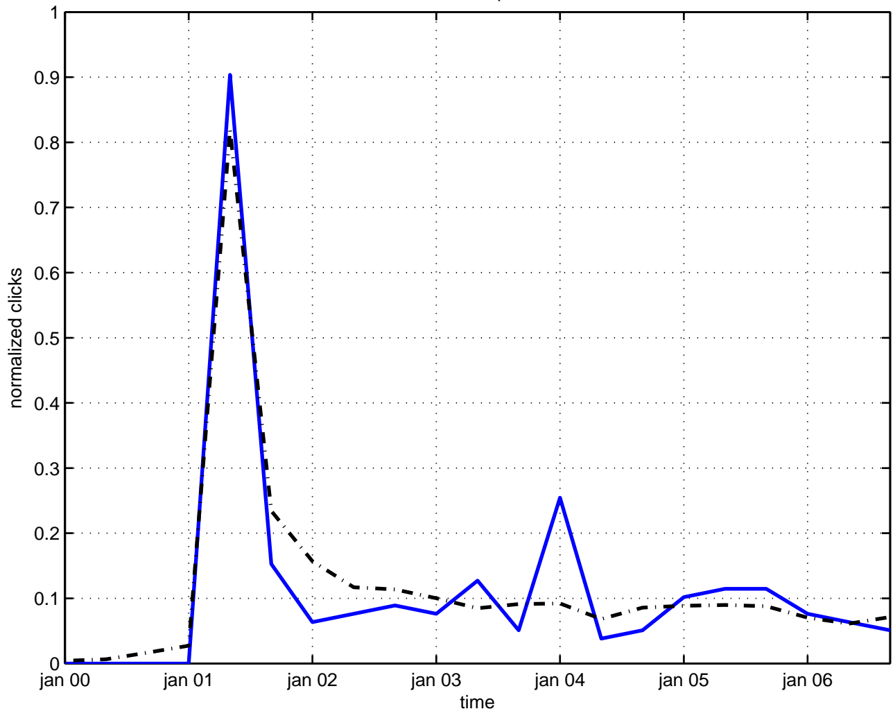
bateman equation
