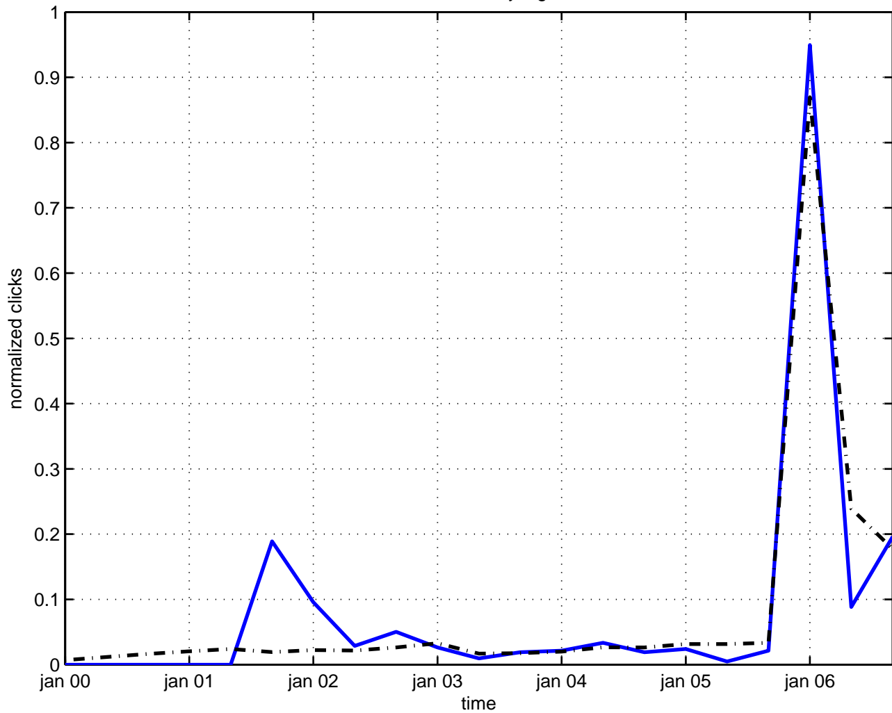
batalin–vilkovisky algebra
