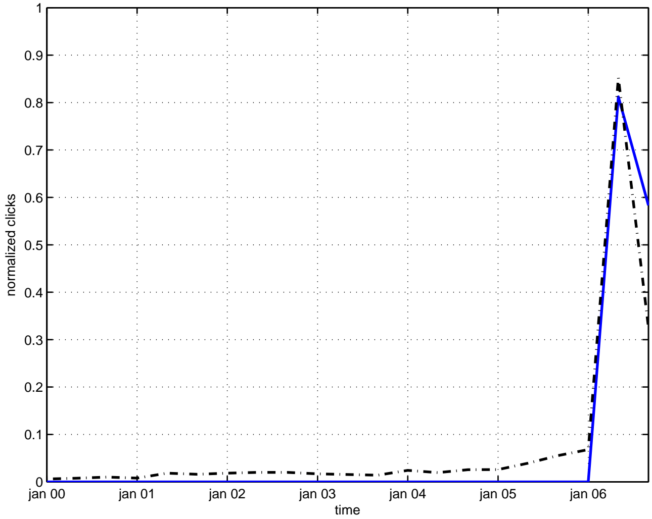
baryogenesis
