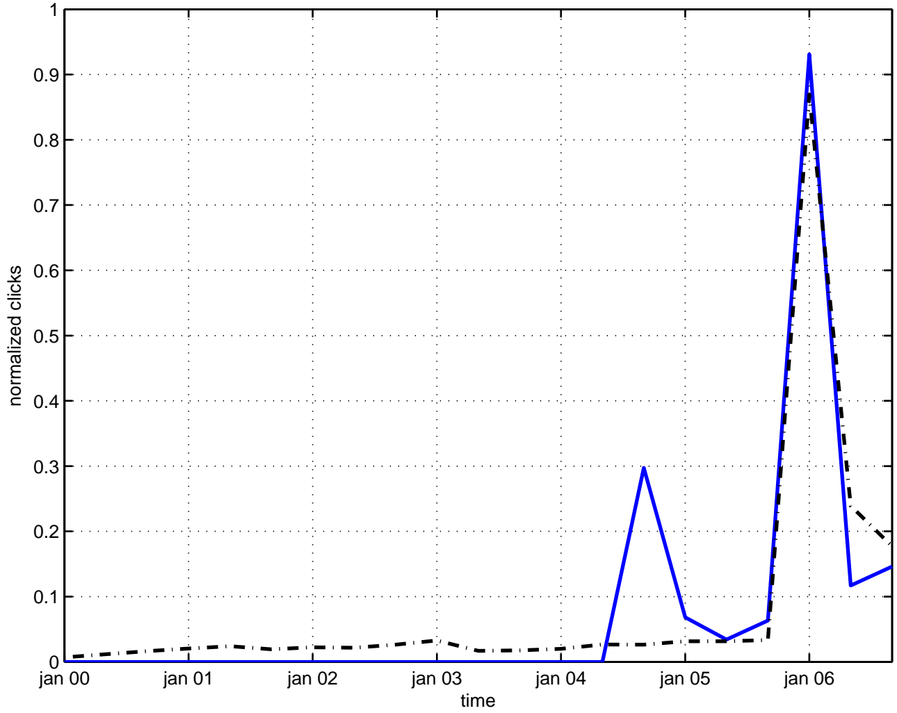
bargmann-wigner equation
