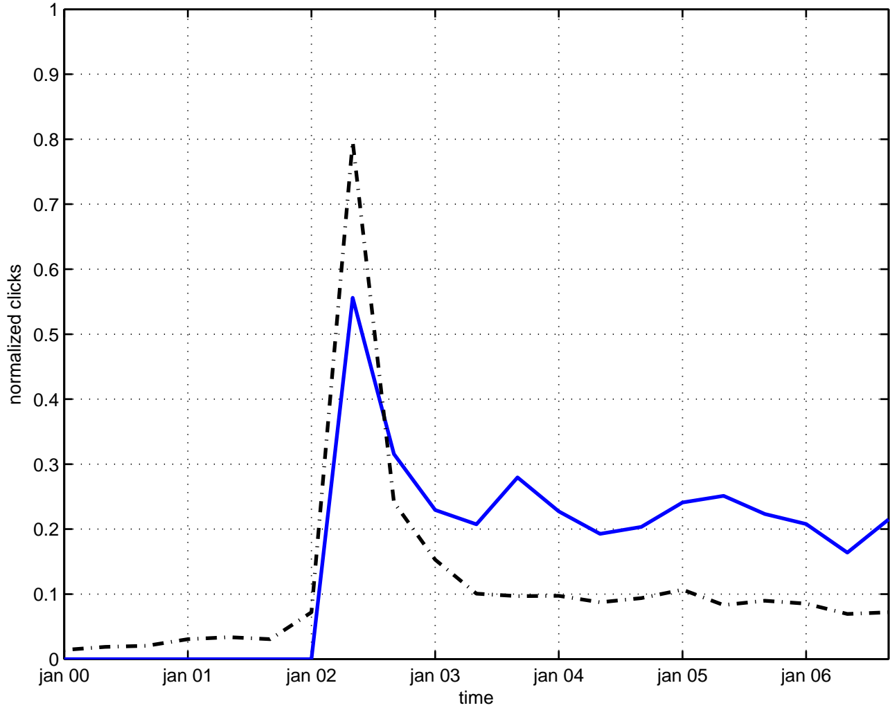
bad honnef 2002/02/25 lectures
