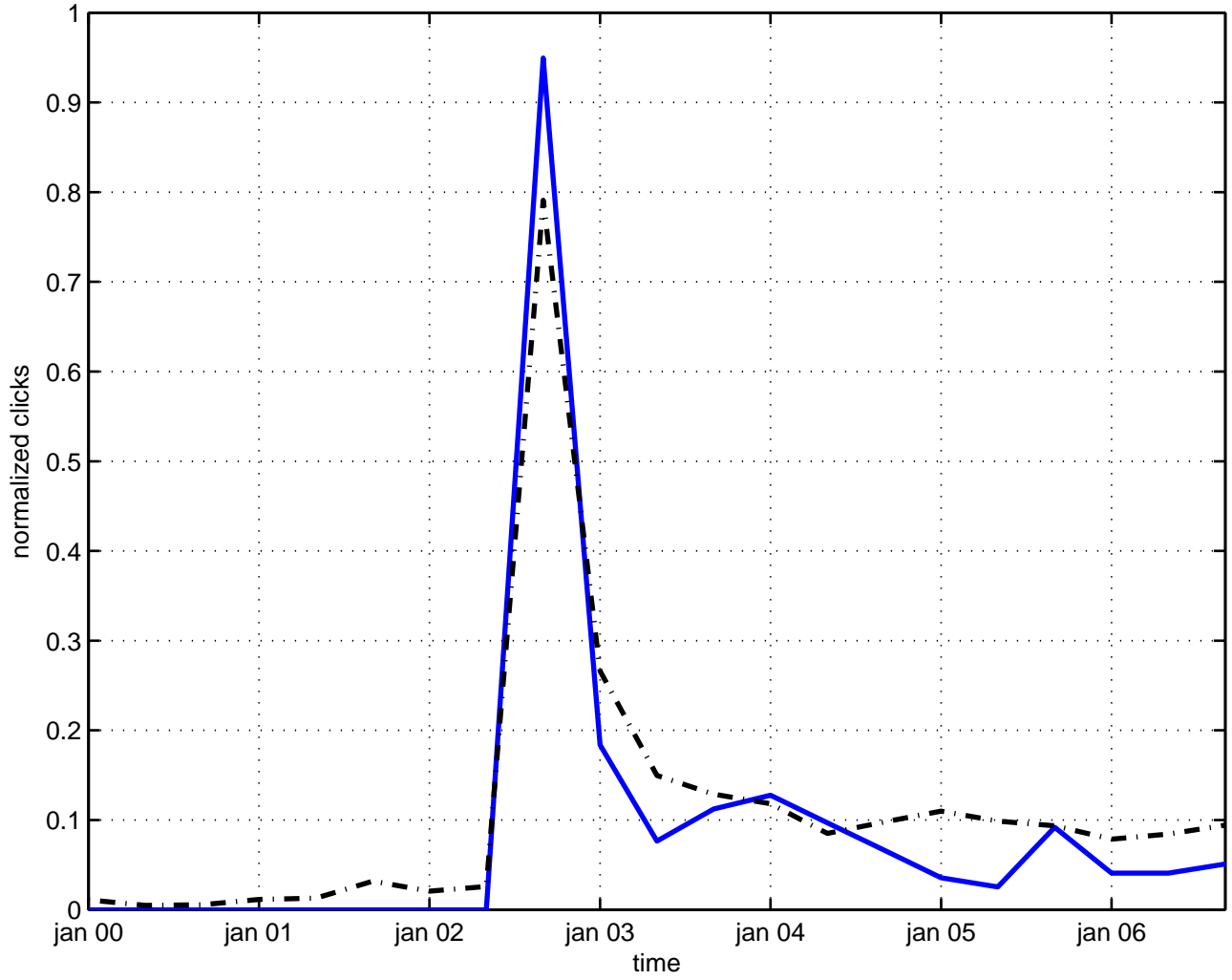
background soliton
