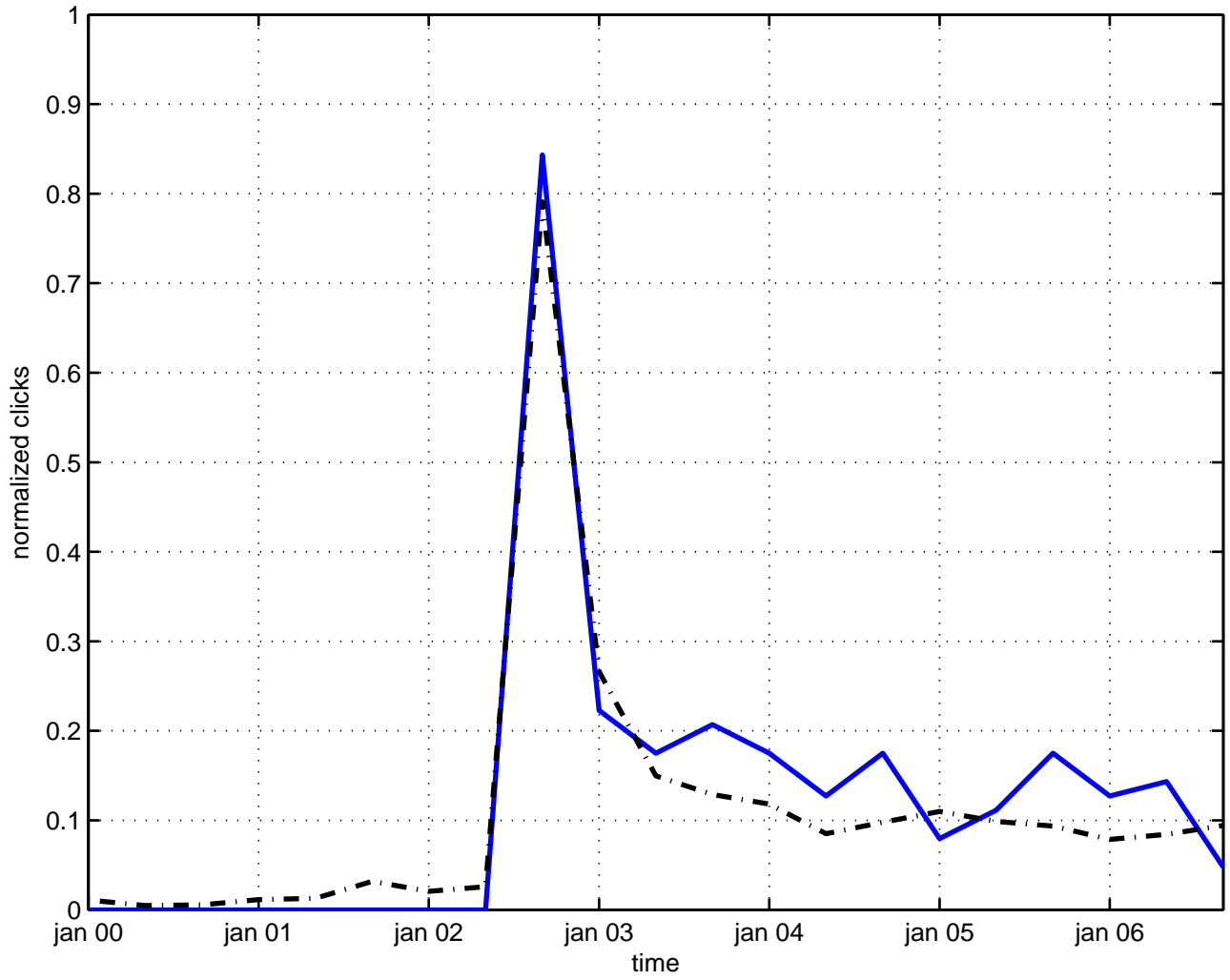
background nucleon
