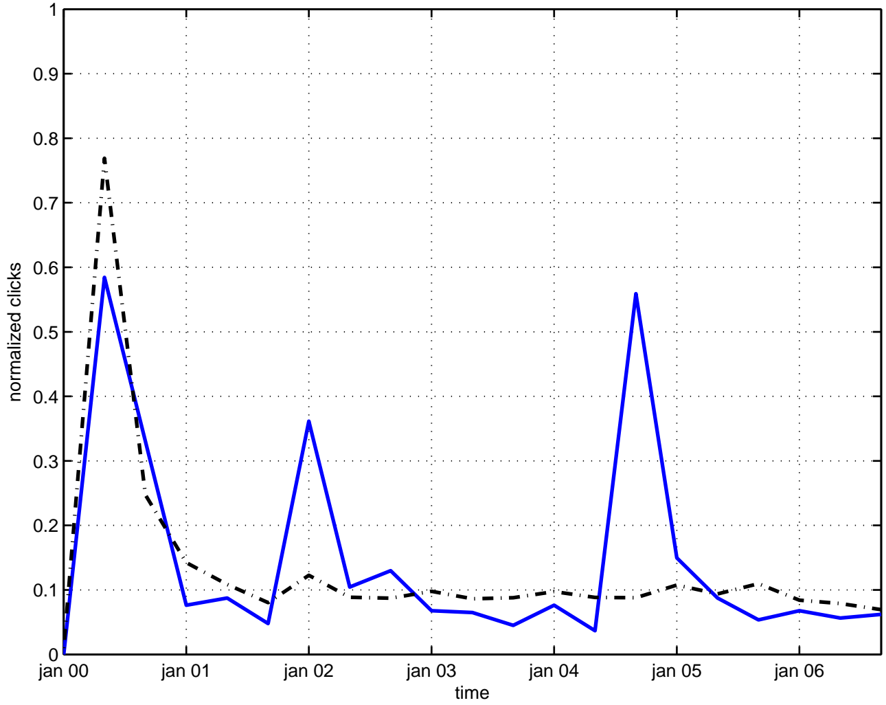
background instanton
