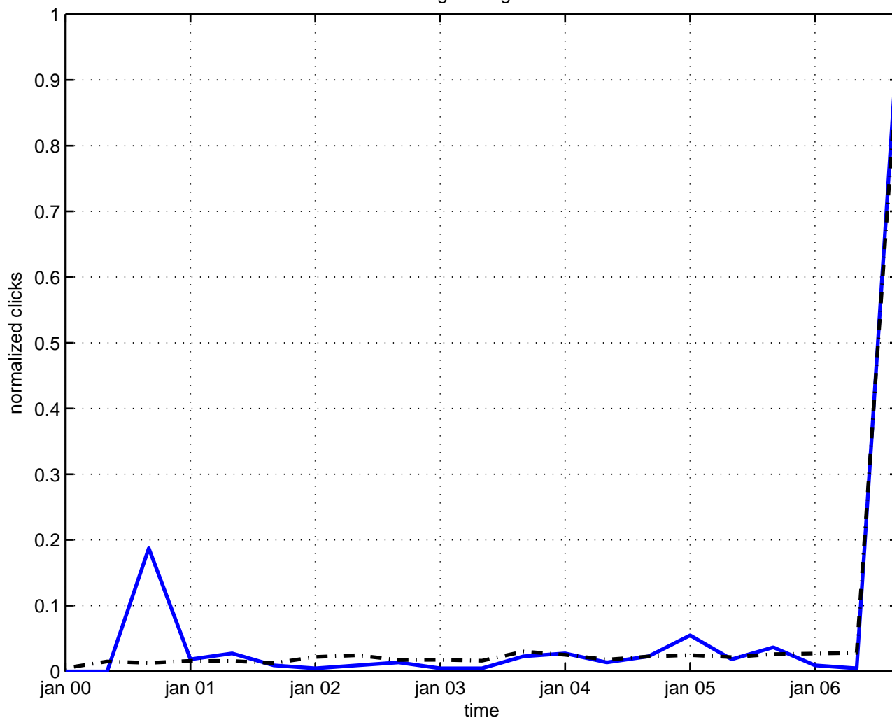
background graviton
