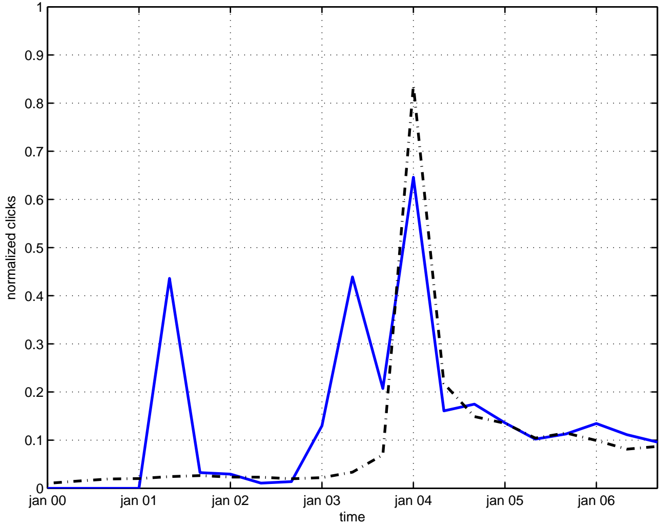
background gravitational radiation
