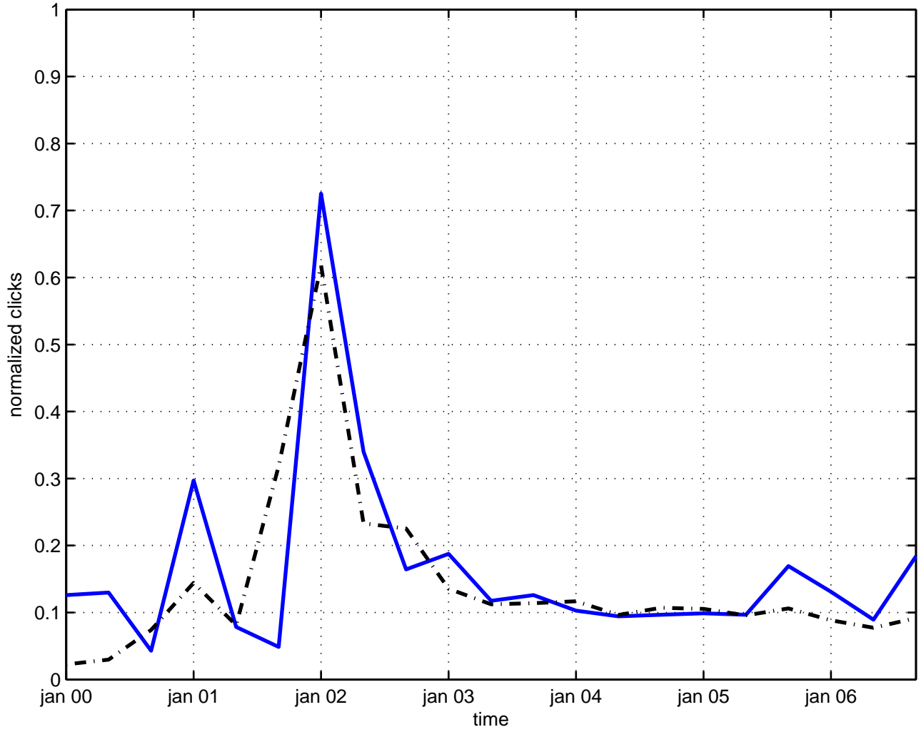
background flux
