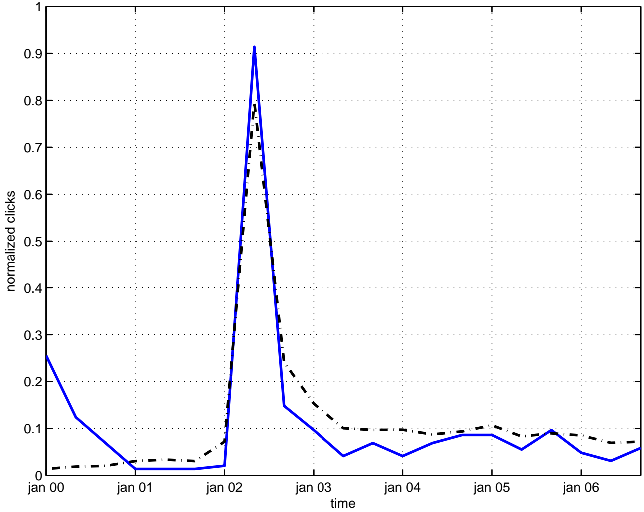
background field string model
