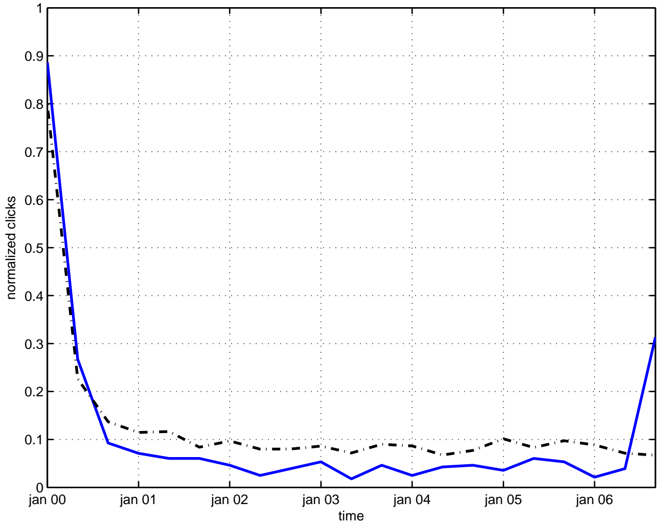
background field magnetic monopole
