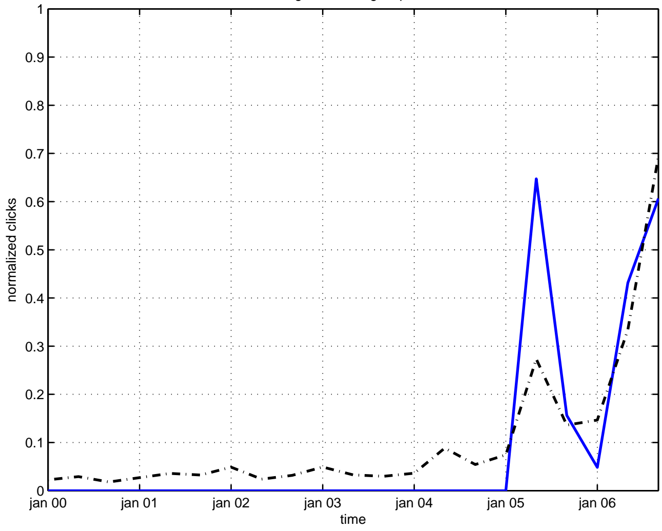
background field graviphoton
