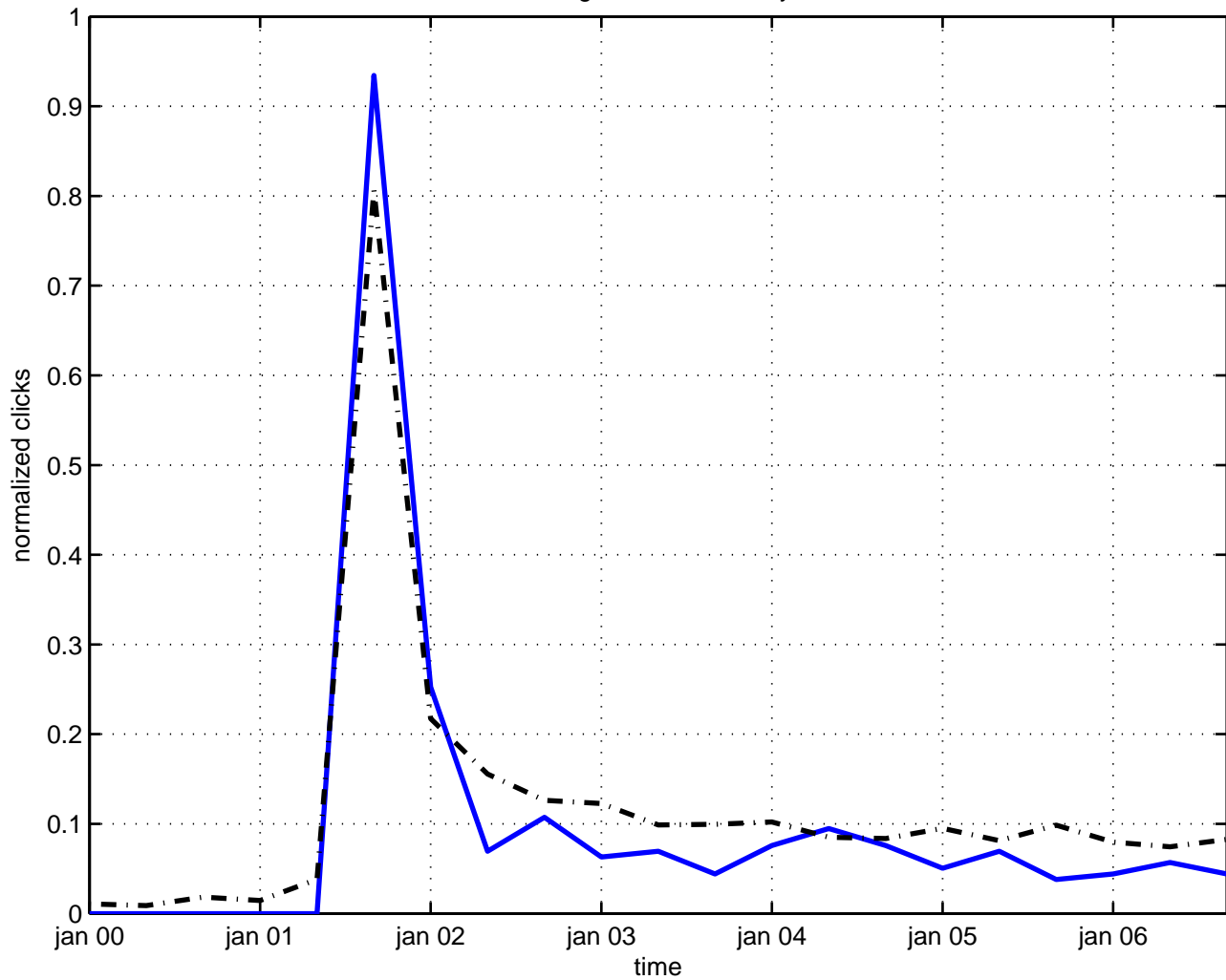
background field duality
