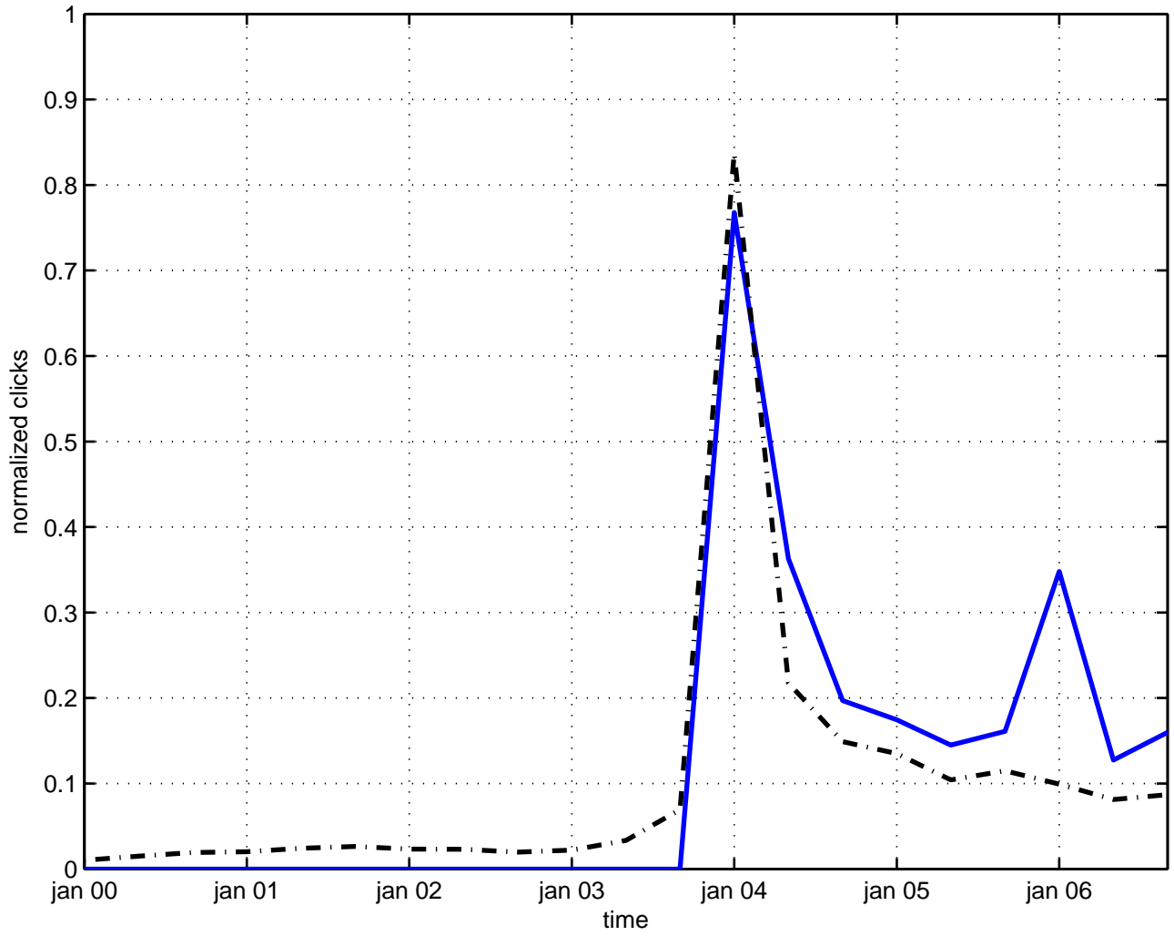
back reaction graviton
