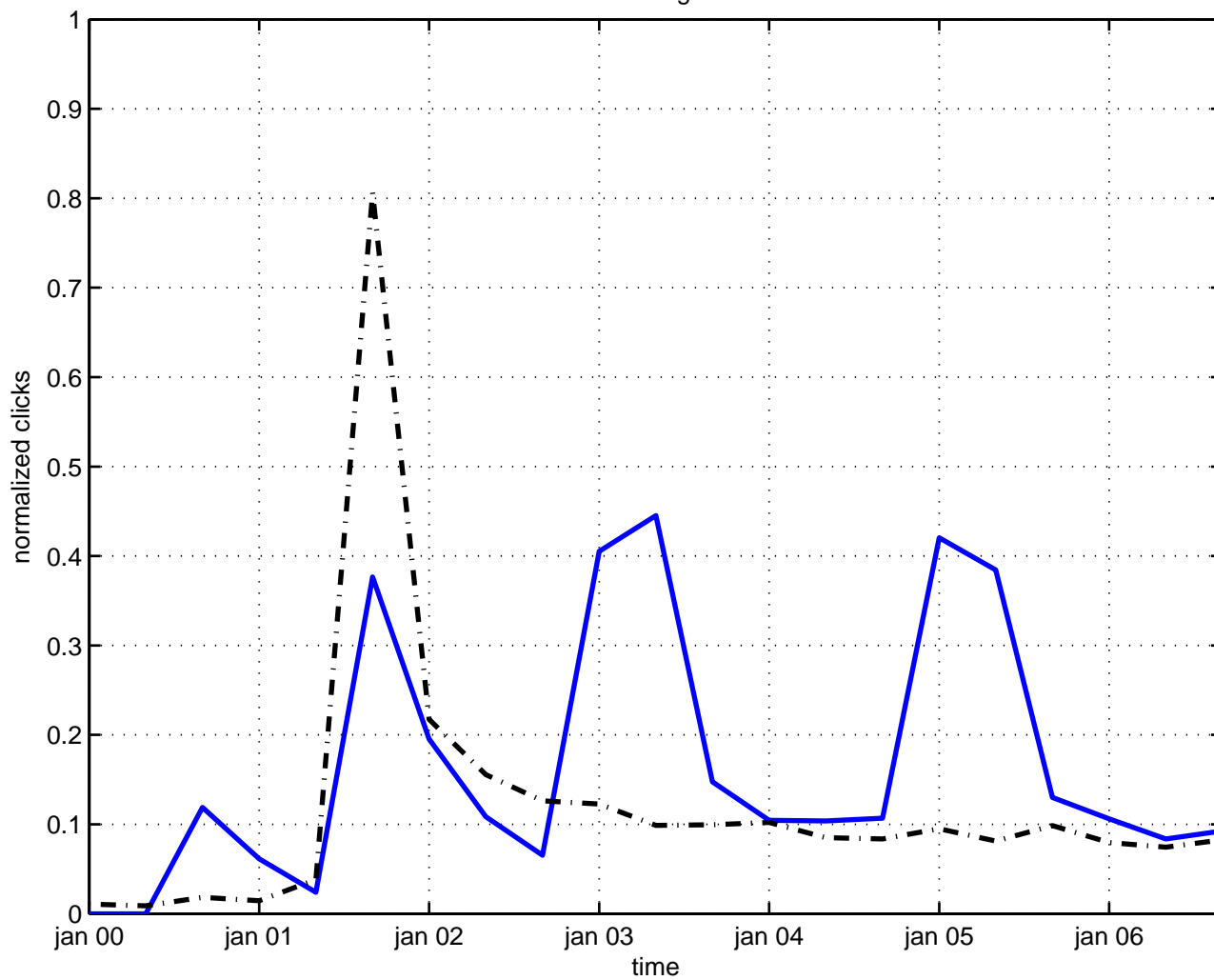
back reaction gravitation
