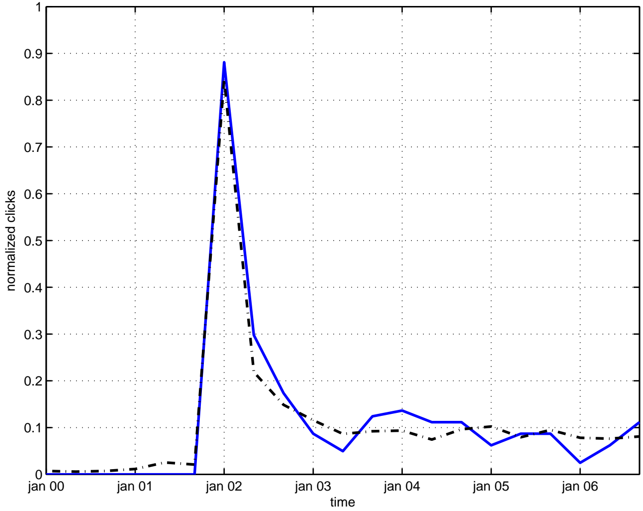
b(2) algebra
