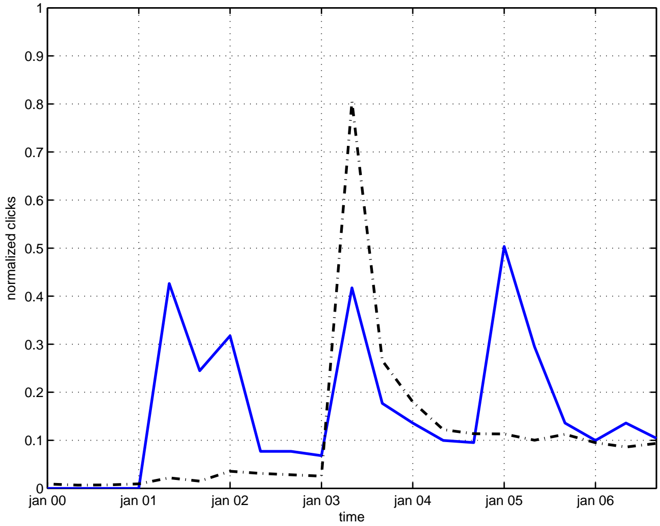
axial-vector current
