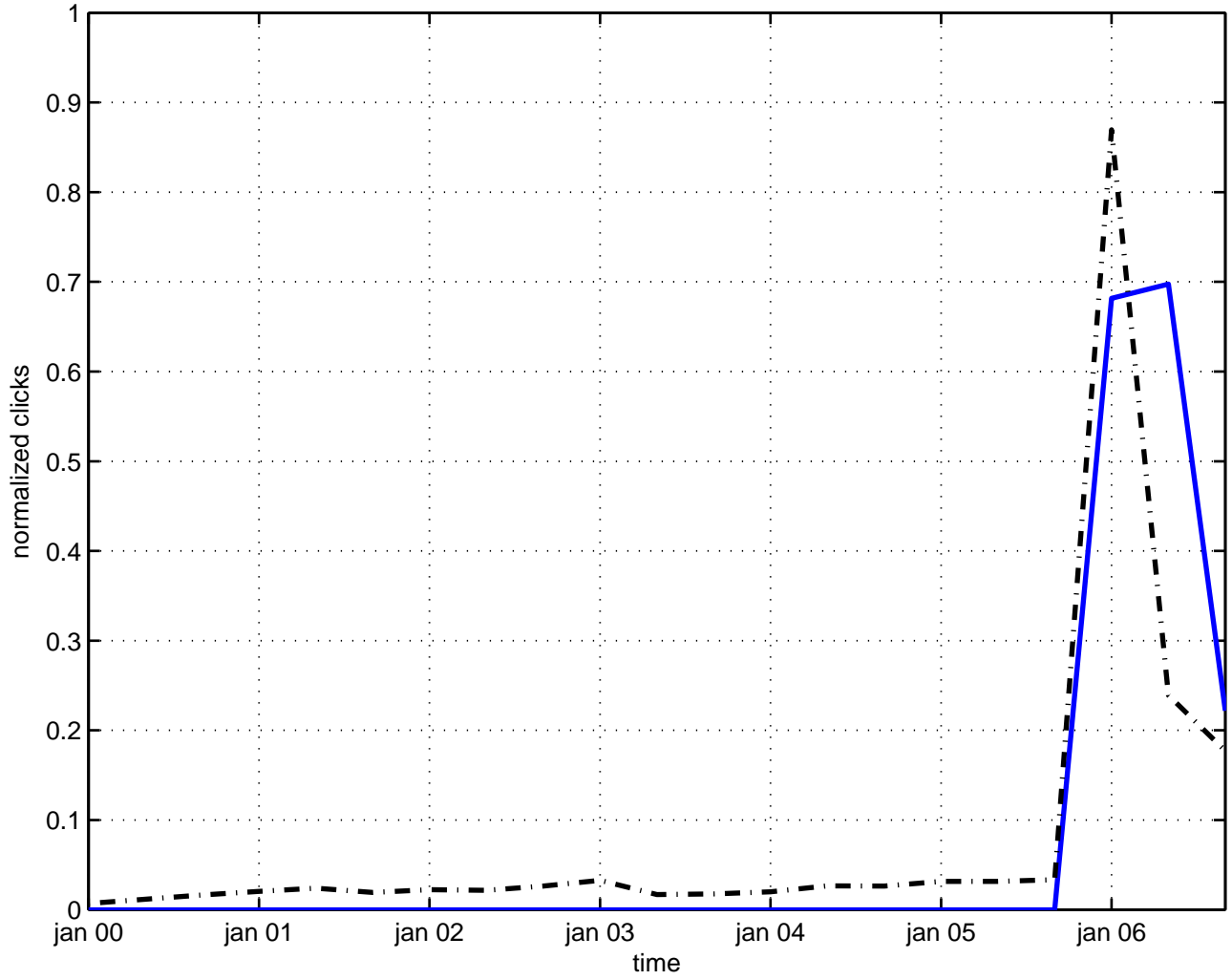
axial-vector background field
