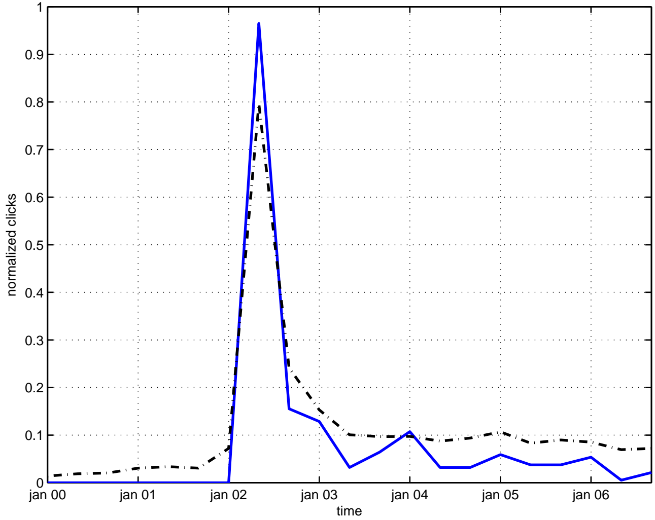
axial gauge field theory
