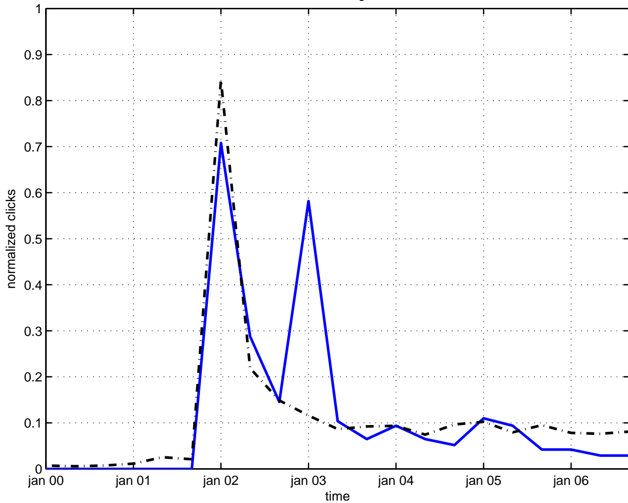
axial charge
