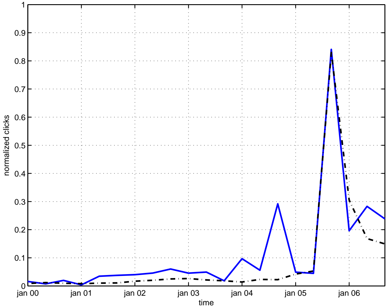
axial anomaly
